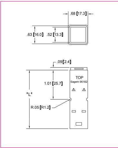
Figure 9. Rod Mount
