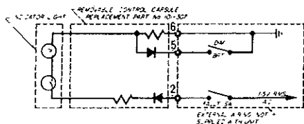
CIRCUIT No. 307 (F307) 115V.A.C. DIM
