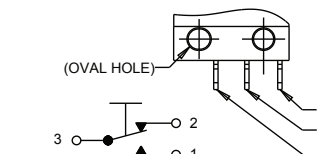
SPDT-FORM C SCHEMATIC CIRCUIT STYLE 3 SPDT, FORM C
