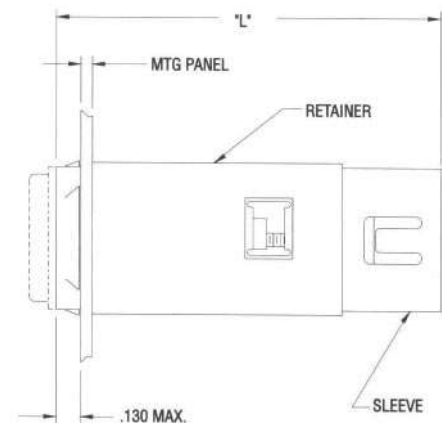
Snap-On Mounting Sleeve
