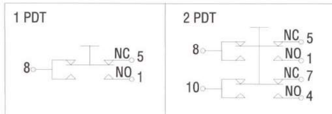
Form "C" Switch Circuits
