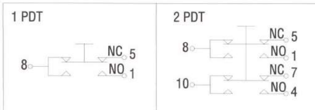
Form "C" Switch Circuits
